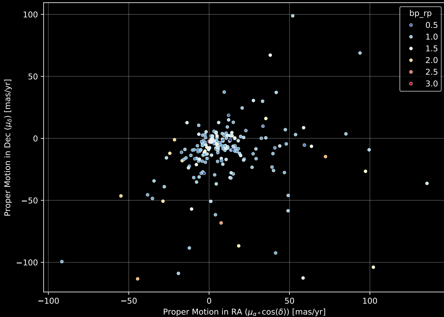
APOGEE DR17 Field: [183-44_MGA] Proper Motion Diagram (n= 205)
