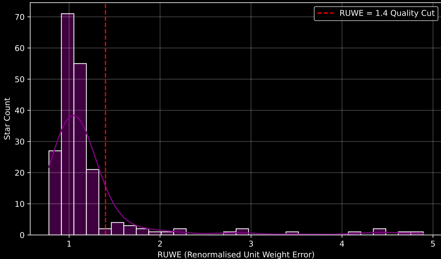
GAPOGEE DR17 Field [183-44_MGA] RUWE Distribution (n= 198)
