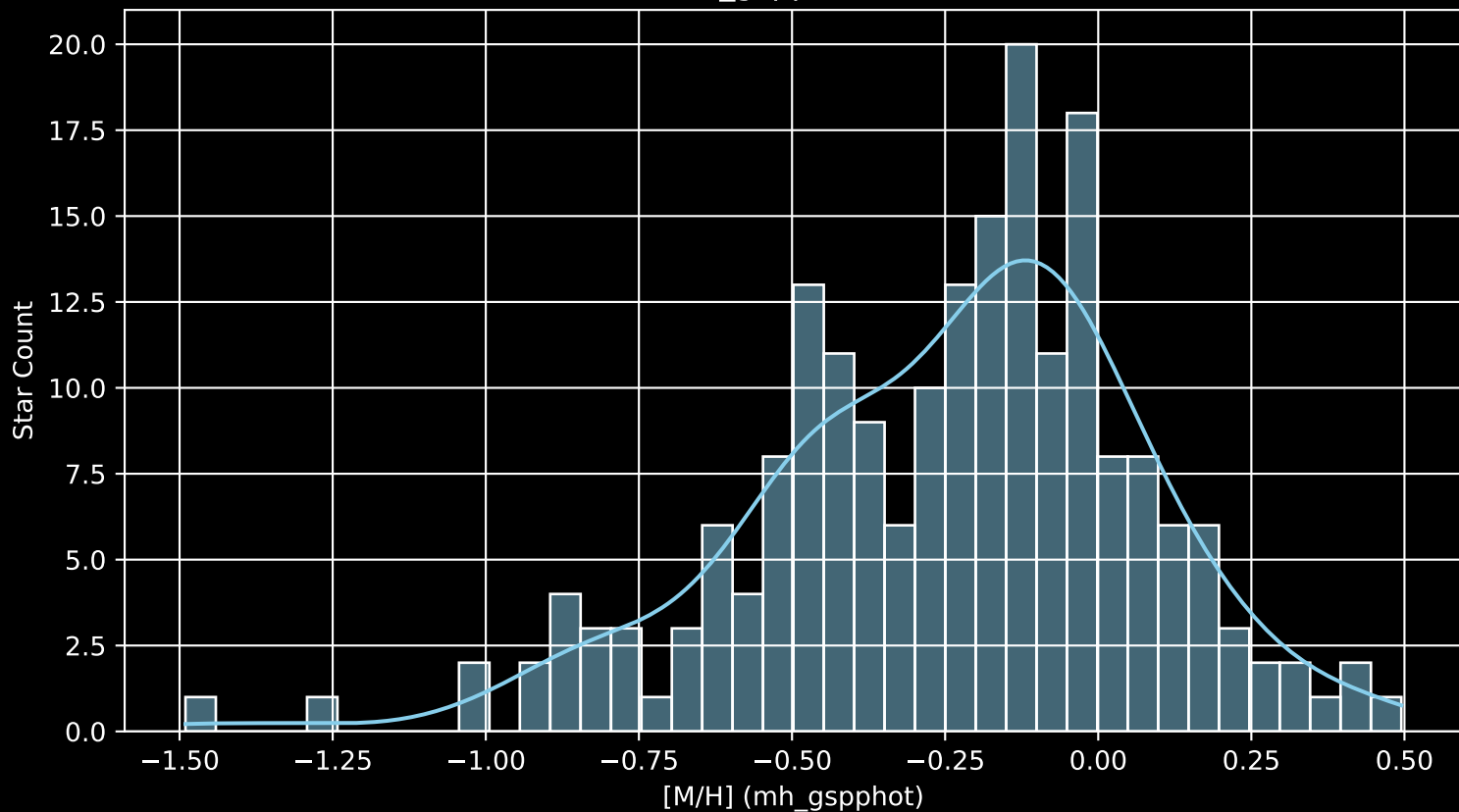
APOGEE DR17 Field: [183-44_MGA [M/H] (mh_gspphot) (n= 203)
