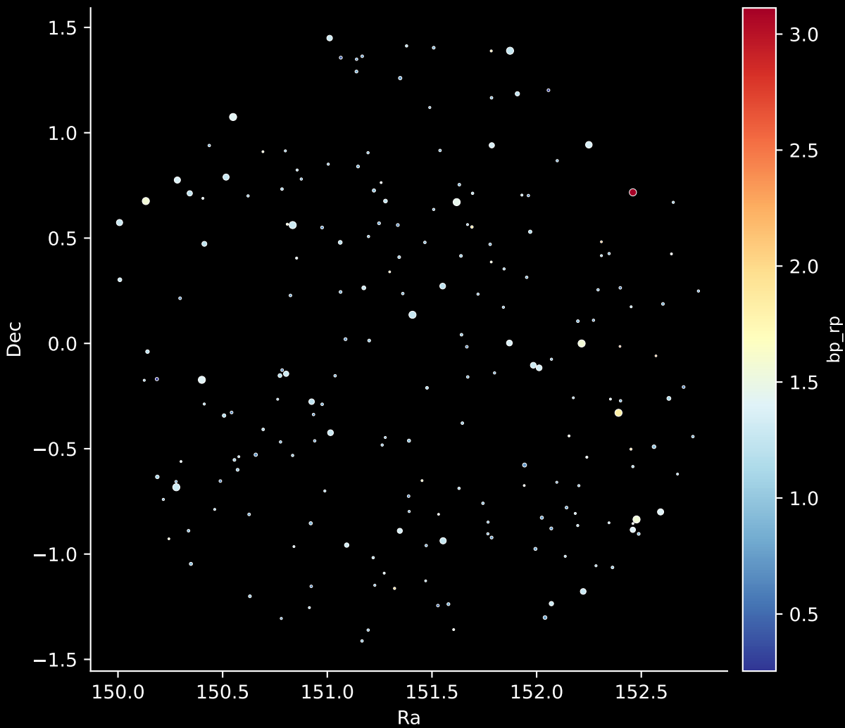
APOGEE DR17 Field: [183-44_MGA] Stars: 205
