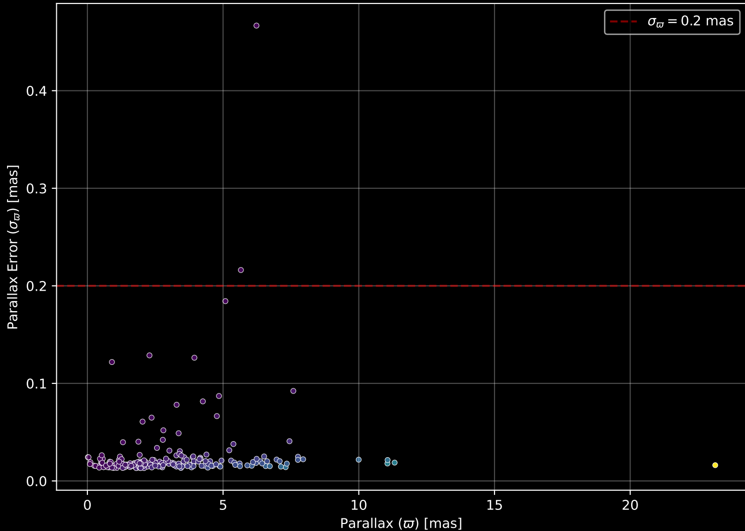
APOGEE DR17 Field: [183-44_MGA] Parallax Quality (n= 205)
