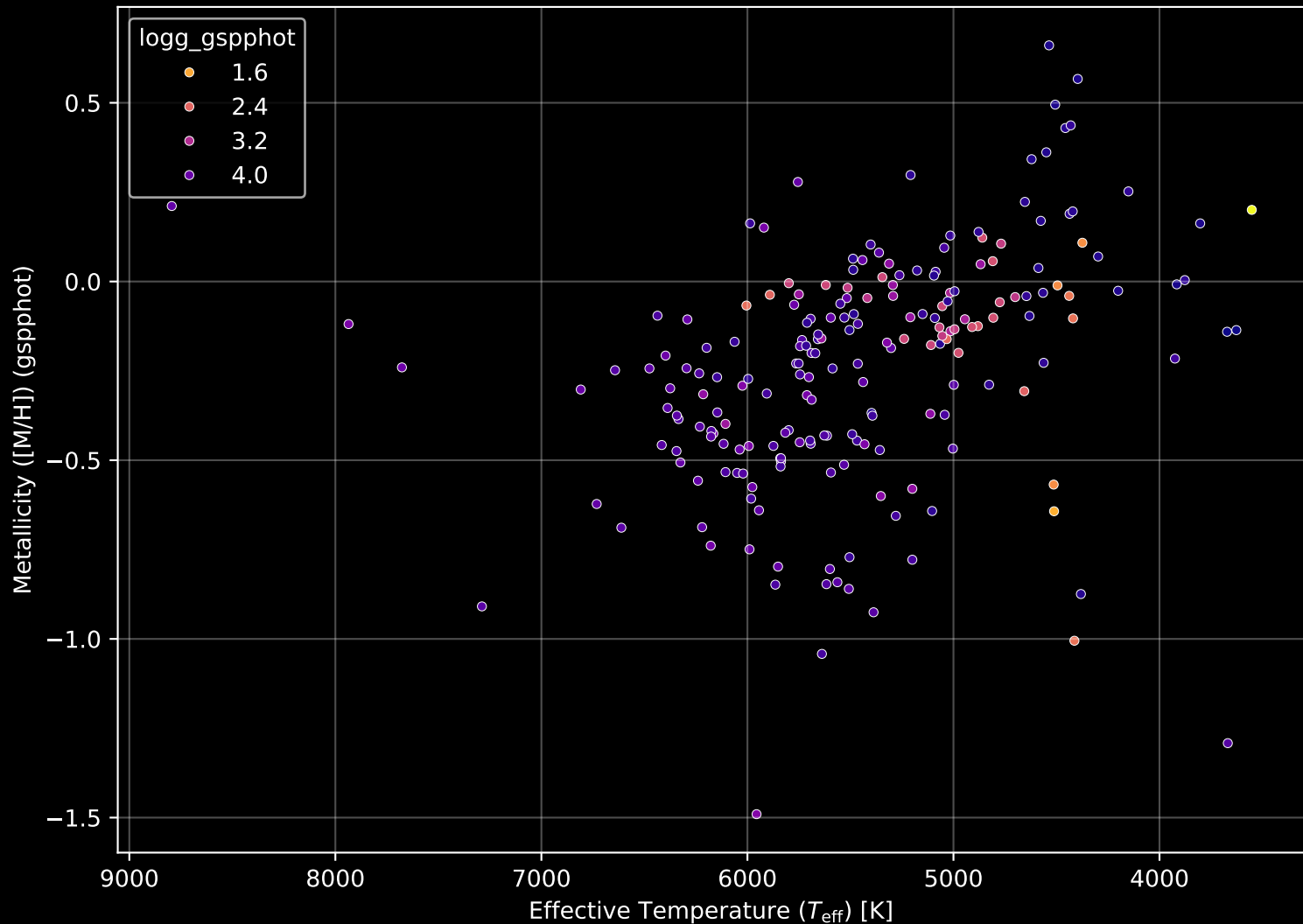
APOGEE DR17 Field: [183-44_MGA] Stellar Population Parameters (n= 205)
